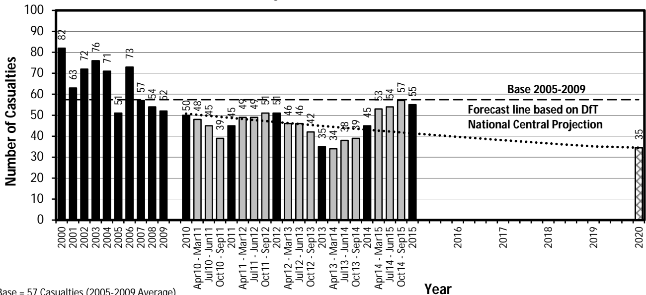
KSI Casualty Trend from 2000 including Annual Data to December 2015 and Projection to 2020, Trafford
