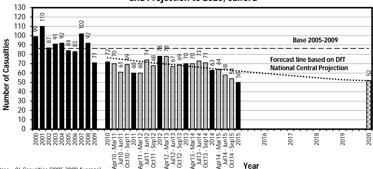
KSI Casualty Trend from 2000 including Annual Data December 2015 and Projection to 2020, Salford
