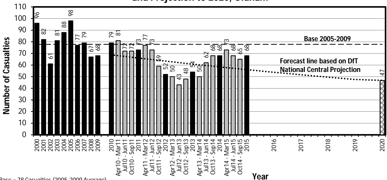
KSI Casualty Trend from 2000 including Annual Data to December 2015 and Projection to 2020, Oldham
