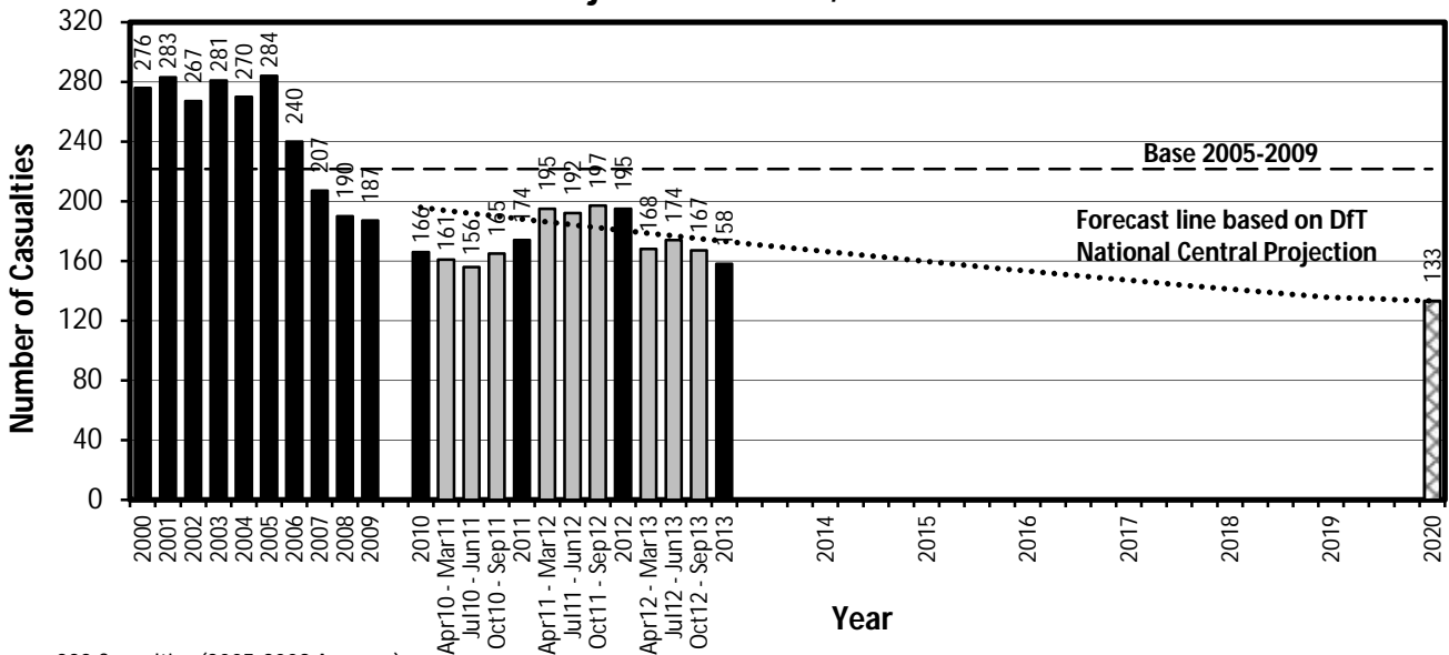
KSI Casualty Trend from 2000 including Annual Data to December 2013 and Projection to 2020, Manchester
