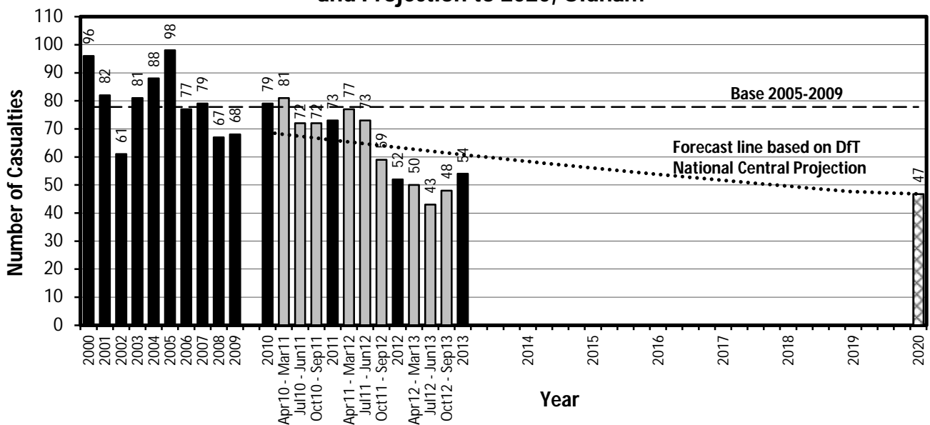
KSI Casualty Trend from 2000 including Annual Data to December 2013 and Projection to 2020, Oldham
